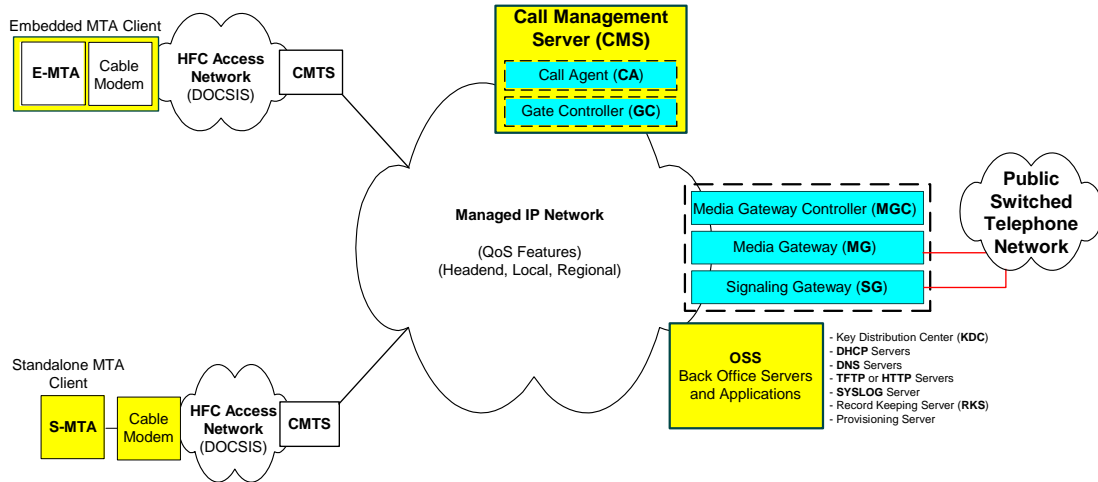
Figure 1. PacketCable Network Component Reference Mode
