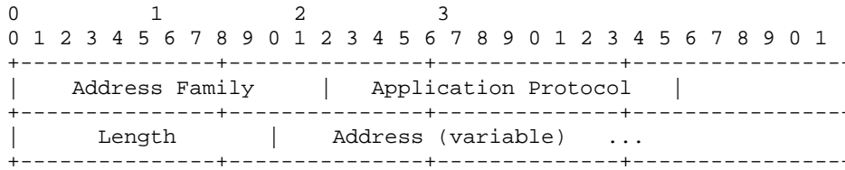
Figure 6–11 - Route Format for WithdrawRoutes and ReachableRoutes
