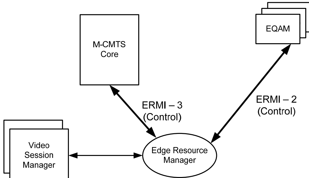
Figure 7-1 - RTSP Client - RTSP Server Relationships
