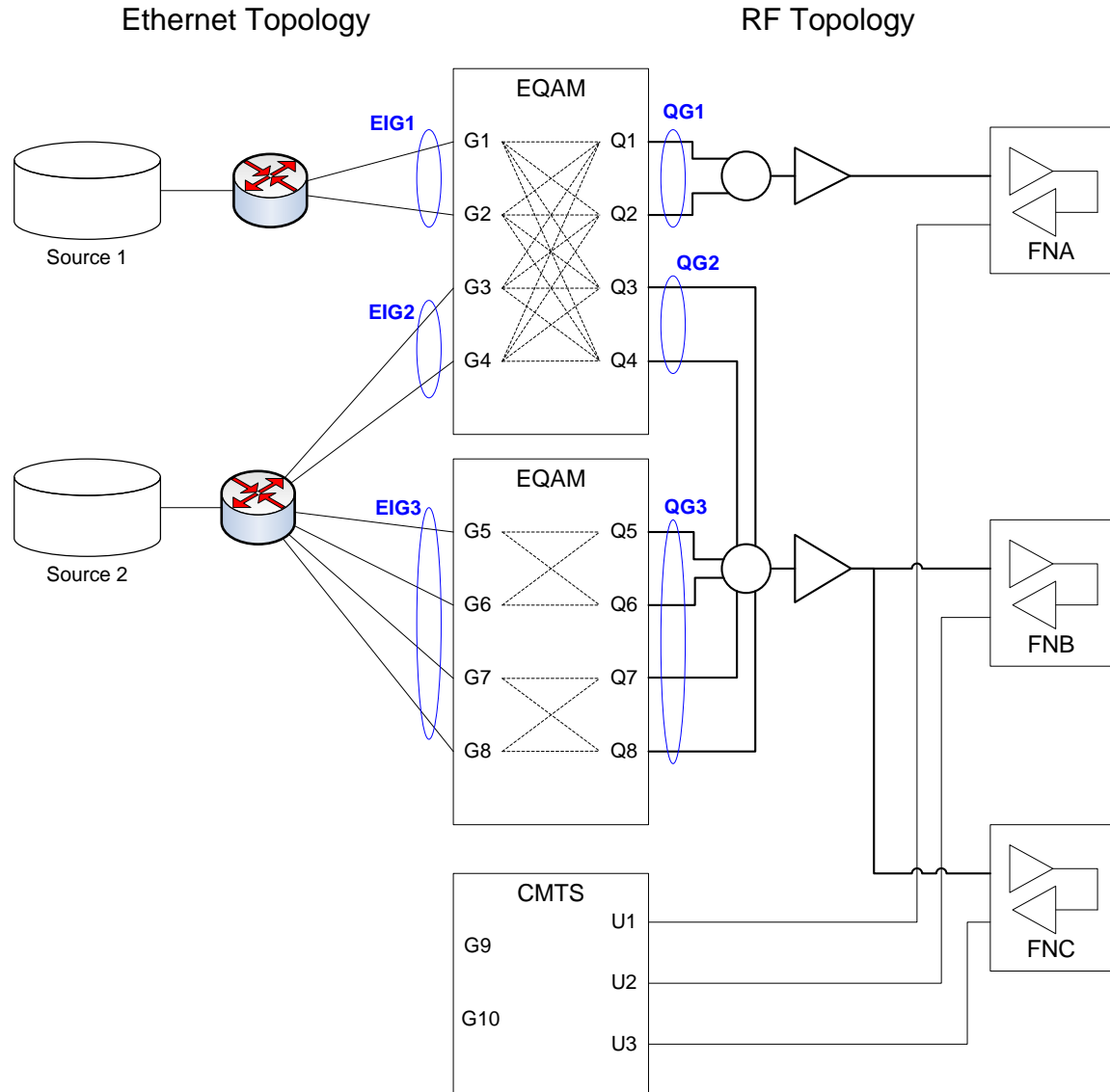
Figure 5–1 - RF Topology
