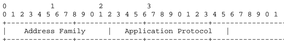
Figure 6-5 - Route Type Format
