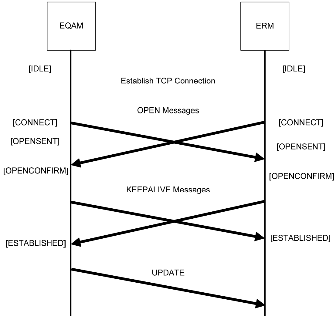
Figure 6-29 - Example ERRP Connection Establishment
