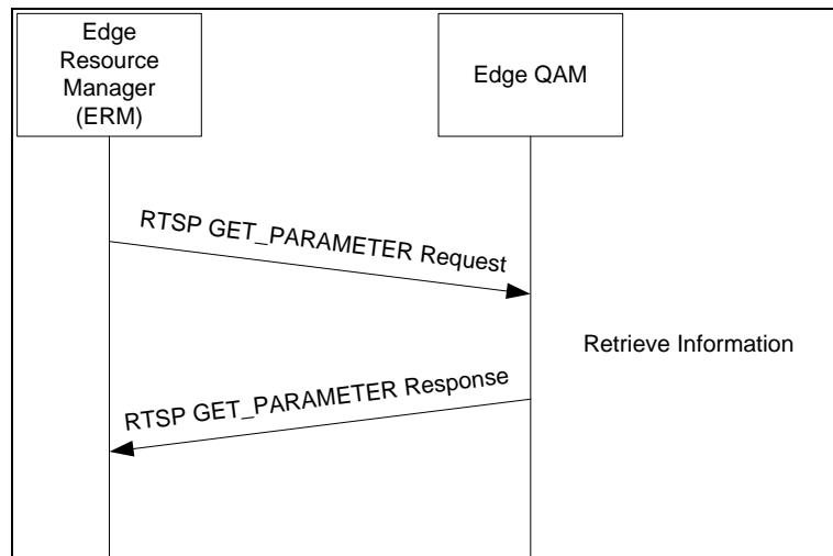
Figure 7-3 - GET_PARAMETER Interaction Diagram
