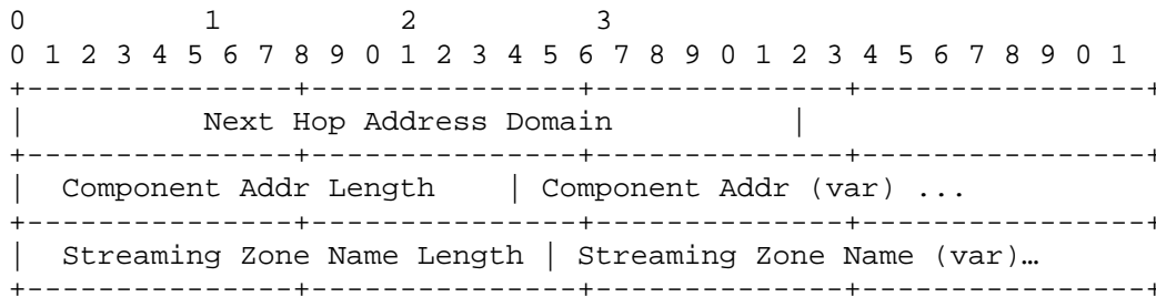
Figure 6–13 - NextHopServer Syntax
