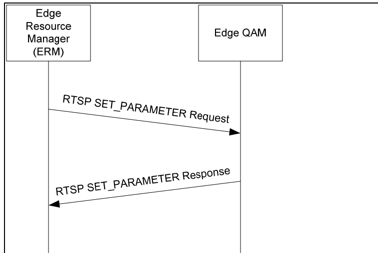
Figure 7-2 - Keepalive Interaction Diagram
