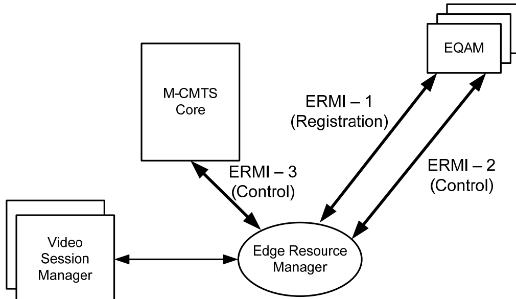
Figure 1-2 - ERMI Interfaces
