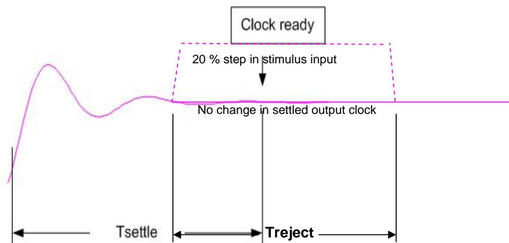
Figure 6-10 - Rejecting impulse noise
