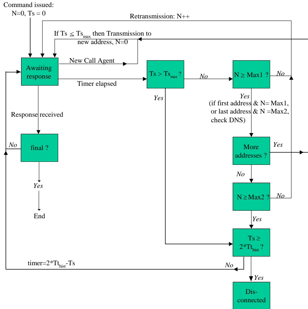
Figure 4 - Retransmission Algorithm
