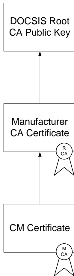
Figure 9-3. CM Certification Chain
