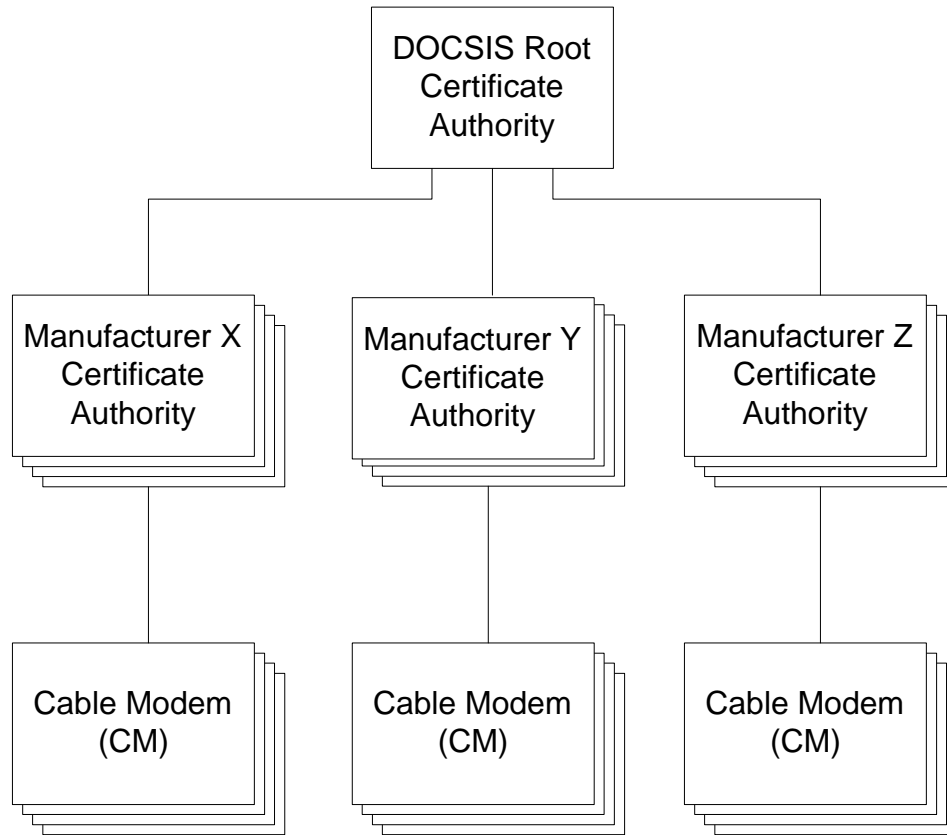
Figure 9-2. The Distributed Model of the DOCSIS Certificate Management Architecture
