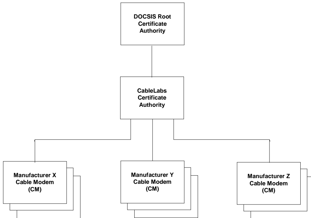
Figure 9-1. The Centralized Model of the DOCSIS Certificate Management Architecture
