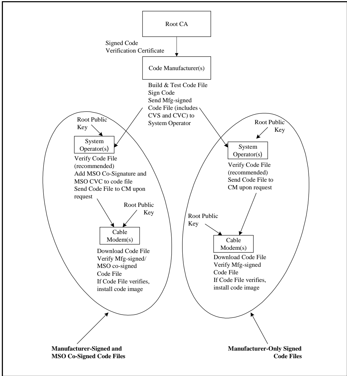
Figure D-1. Typical Code Validation Hierarchy
