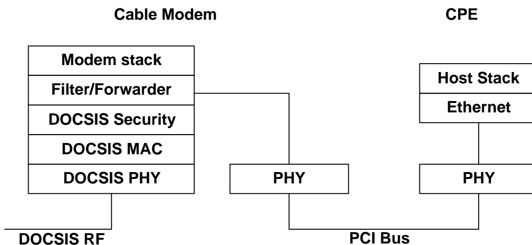
Figure 3-7 CM-to-PC Forwarding
