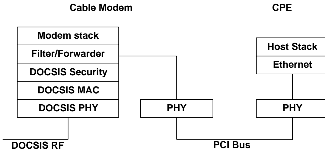
Figure 3-9 CM-to-MAC Forwarding
